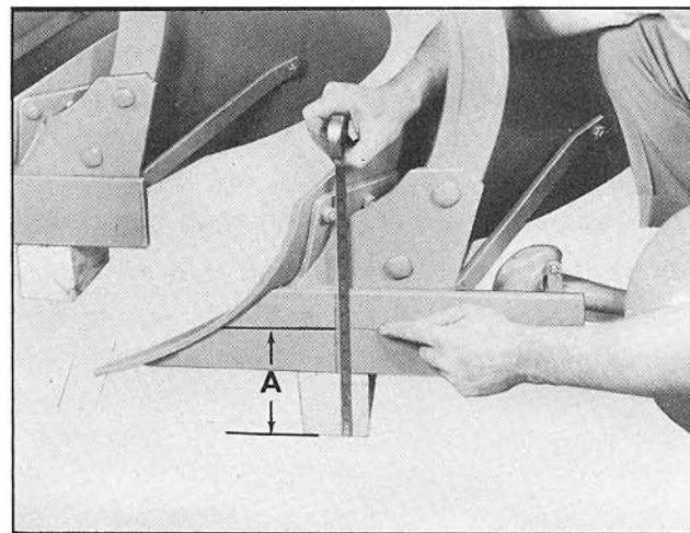
Fig. 16 Dimension "A"
