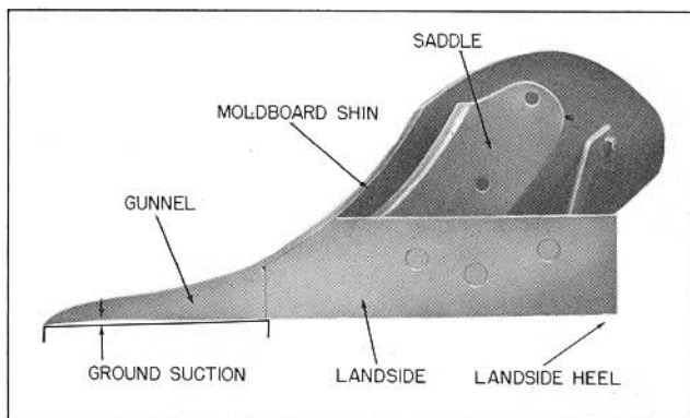
Fig. 13 Ground Suction
