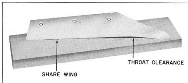
Fig. 12 Throat Clearance
