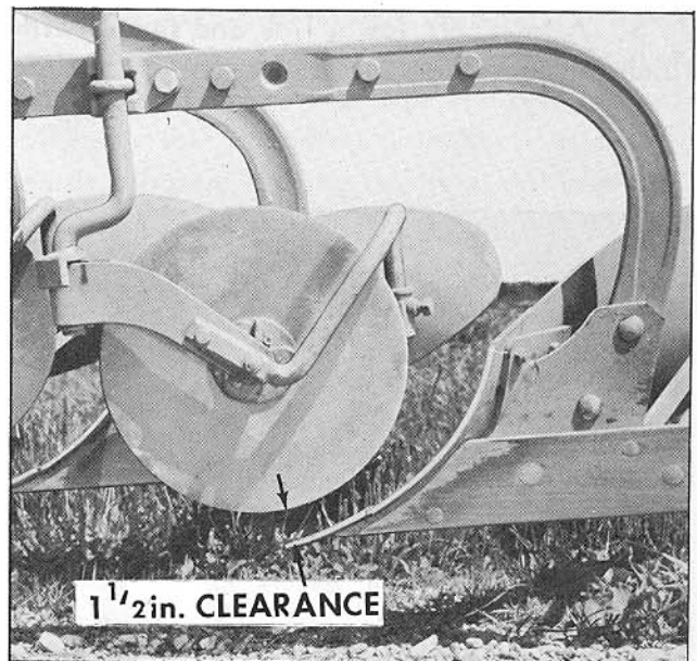
Fig. 6 Coulters Setting
