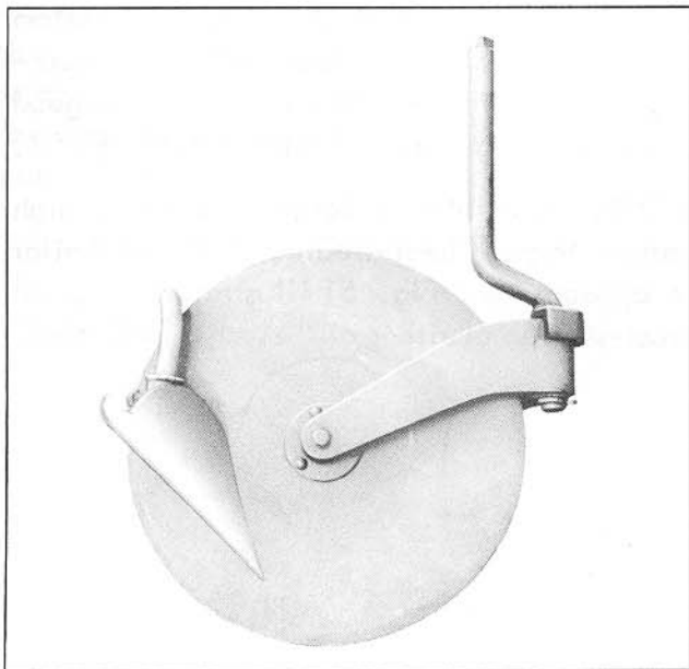
Fig. 53 Plain Rolling Coulter
